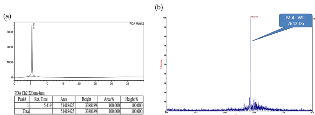
Figure 7.2 (a) HPLC-chromatogram and (b) Mass spectrum of mPNC-NLS (Peptide sequence: QETFSDLWKLLVQRKRQKLMP).
