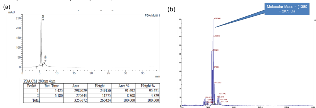
Figure 7.3 (a) HPLC-chromatogram and (b) Mass spectrum of mPNC (Peptide sequence: QETFSDLWKLL).
