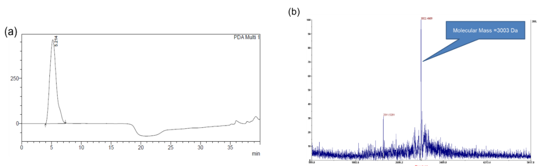
Figure 7.4 (a) HPLC-chromatogram and (b) Mass spectrum of fluorescein attached mPNC-NLS (Peptide sequence: Fluorescein-QETFSDLWKLLVQRKRQKLMP).
