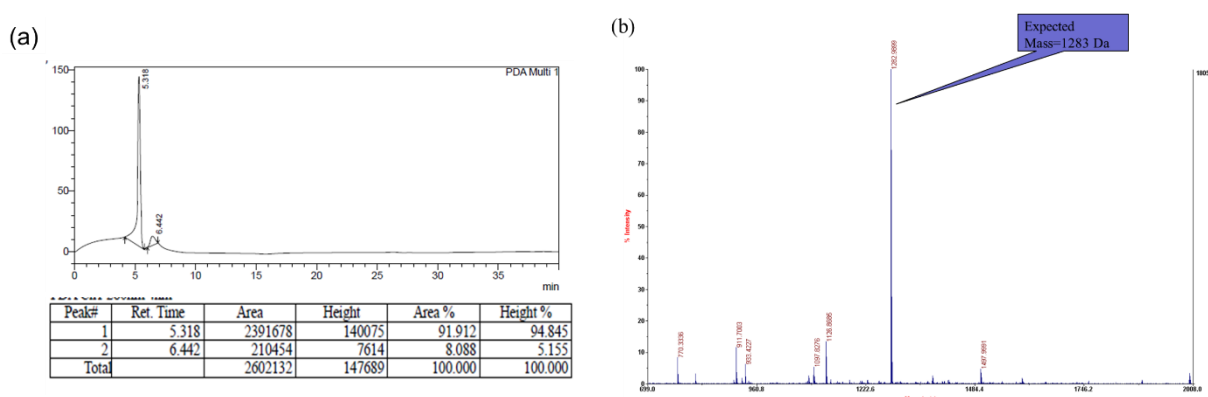
Figure 7.5 (a) HPLC-chromatogram and (b) Mass spectrum of fluorescein attached mPNC (Peptide sequence: Fluorescein-QETFSDLWKLL).
